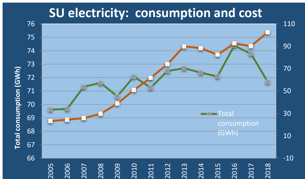
Figure 6: Electricity consumption and cost at SU, 2005 to 2018
