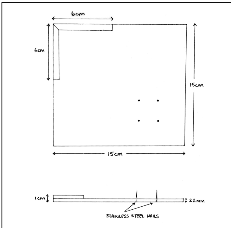
Imilinganiselo neenkcukacha zobucukubhode zebhodi yokuqabela nokuxobulela
