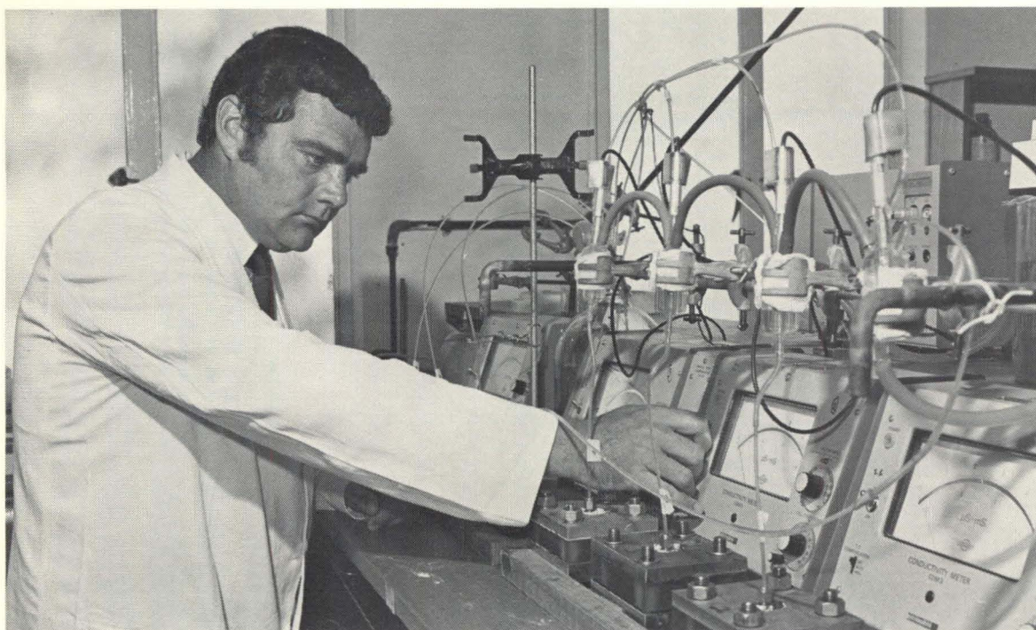
Dr Derik Pienaar measuring permeate salinity on an automatic reverse osmosis apparatus.
